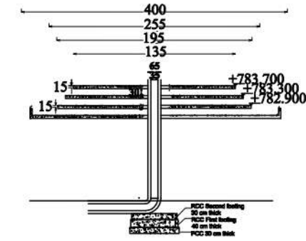
AERATOR SECTION
