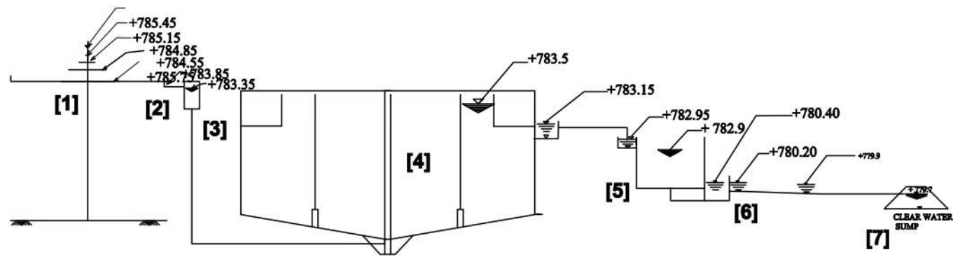
HYDRAULIC FLOW DIAGRAM
